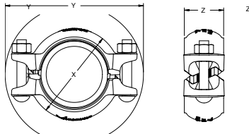
STYLE 177 PRE-ASSEMBLED (INSTALLATION-READY CONDITION)
