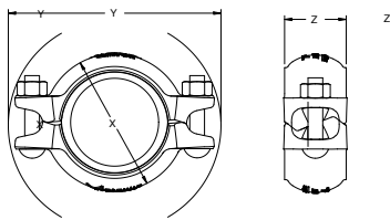
STYLE 177 JOINT ASSEMBLED
